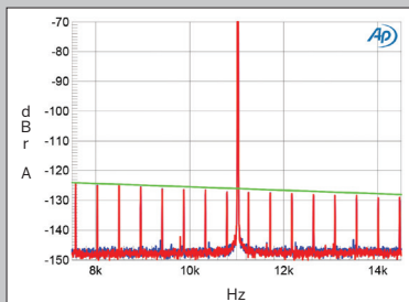
Fig.11 MBL N31, high-resolution jitter spectrum of analog output signal, 11.025kHz at -6dBFS, sampled at 44.1kHz with LSB toggled at 229Hz: 16-bit AES/EBU data (left channel blue, right red). Center frequency of trace, 11.025kHz; frequency range, ±3.5kHz.
