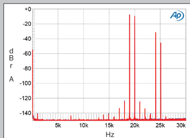
Fig.10 MBL N31, Min filter, HF intermodulation spectrum, DC-30kHz, 19+20kHz at 0dBFS into 600 ohms, 44.1kHz data (left channel blue, right red; linear frequency scale).
