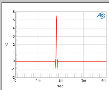
Fig.2 MBL N31, Slow filter, impulse response (one sample at 0dBFS, 44.1kHz sampling, 4ms time window).
