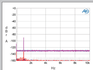
Fig.7 MBL N31, spectrum with noise and spurs of dithered 1kHz tone at -90dBFS with: 16-bit data (left channel cyan, right magenta), 24-bit data (left blue, right red) (20dB/vertical div.).
