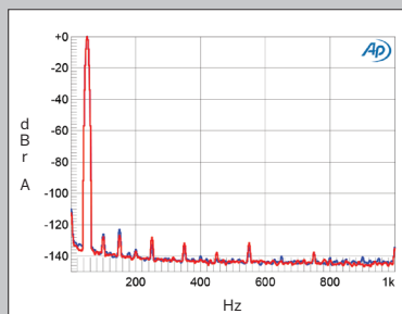
Fig.9 MBL N31, spectrum of 50Hz sinewave, DC-1kHz, at 0dBFS into 600 ohms (left channel blue, right red; linear frequency scale).
