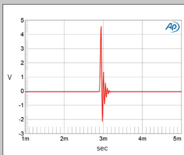
Fig.3 MBL N31, Min filter, impulse response (one sample at 0dBFS, 44.1kHz sampling, 4ms time window).
