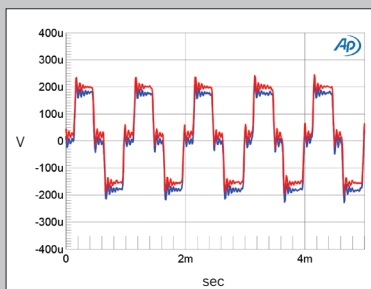
Fig.8 MBL N31, waveform of undithered 1kHz sinewave at -90.31dBFS, 16-bit TosLink data (left channel blue, right red).
