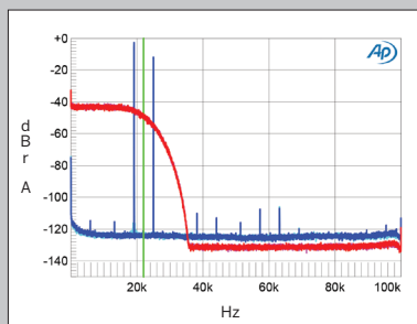
Fig.4 MBL N31, Slow filter, wideband spectrum of white noise at -4dBFS (left channel red, right magenta) and 19.1kHz tone at 0dBFS (left blue, right cyan), with data sampled at 44.1kHz (20dB/vertical div.).
