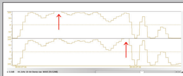
Fig.12 Steely Dan's "Gaslighting Abbie," sample-level waveform display. Red arrows indicate consecutive samples at 0dBFS that would result in intersample overs.
