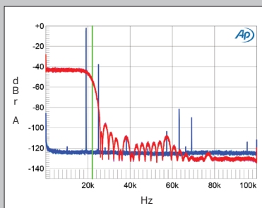
Fig.5 MBL N31, Min filter, wideband spectrum of white noise at -4dBFS (left channel red, right magenta) and 19.1kHz tone at 0dBFS (left blue, right cyan), with data sampled at 44.1kHz (20dB/vertical div.).
